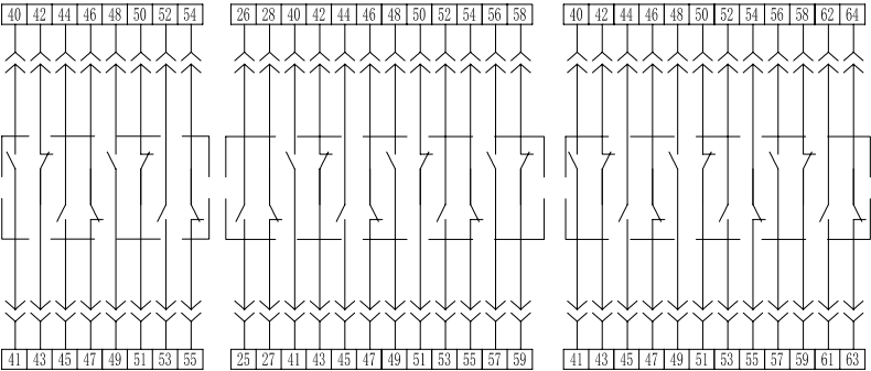
D4-独立4开4闭
