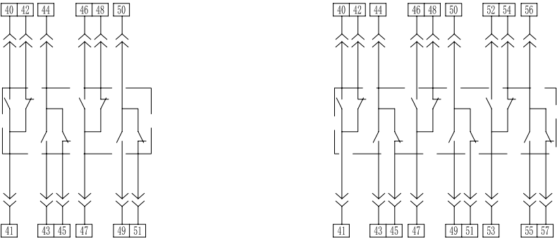
T4-转换4开4闭
